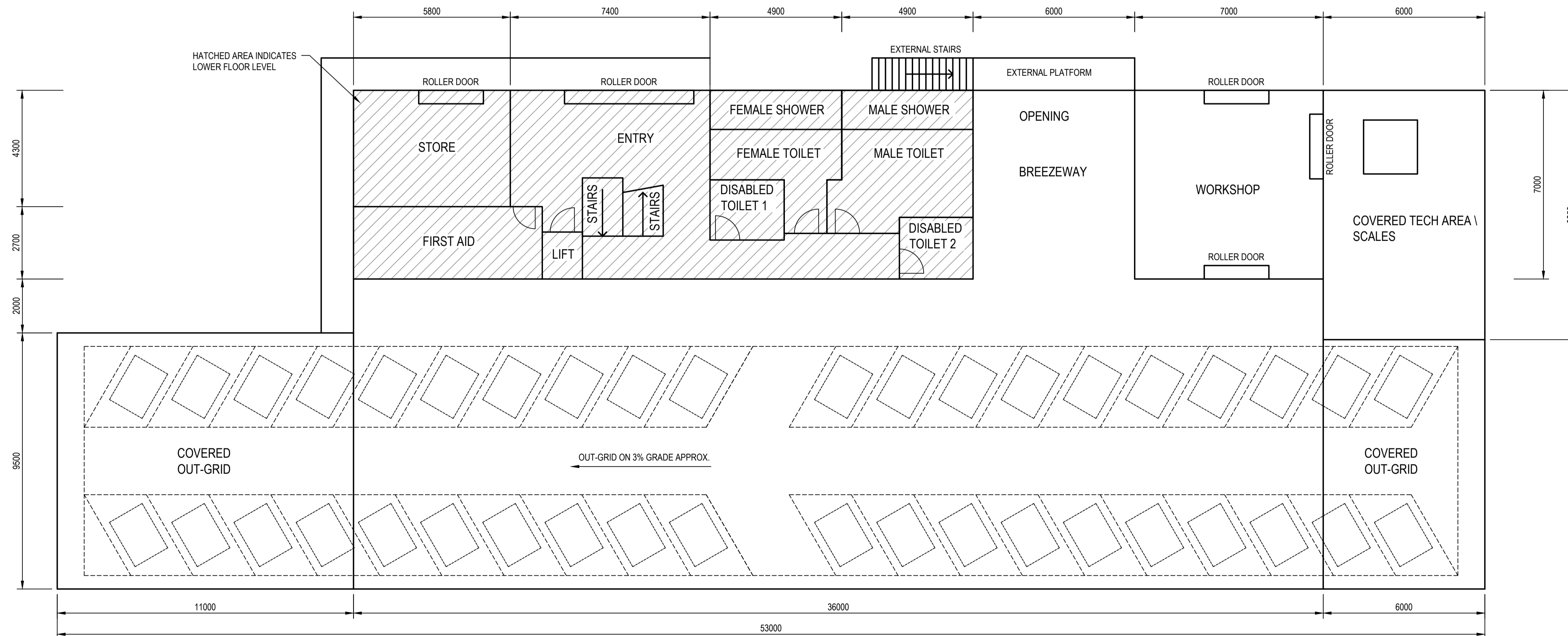
GROUND FLOOR - GENERAL ARRANGEMENT
