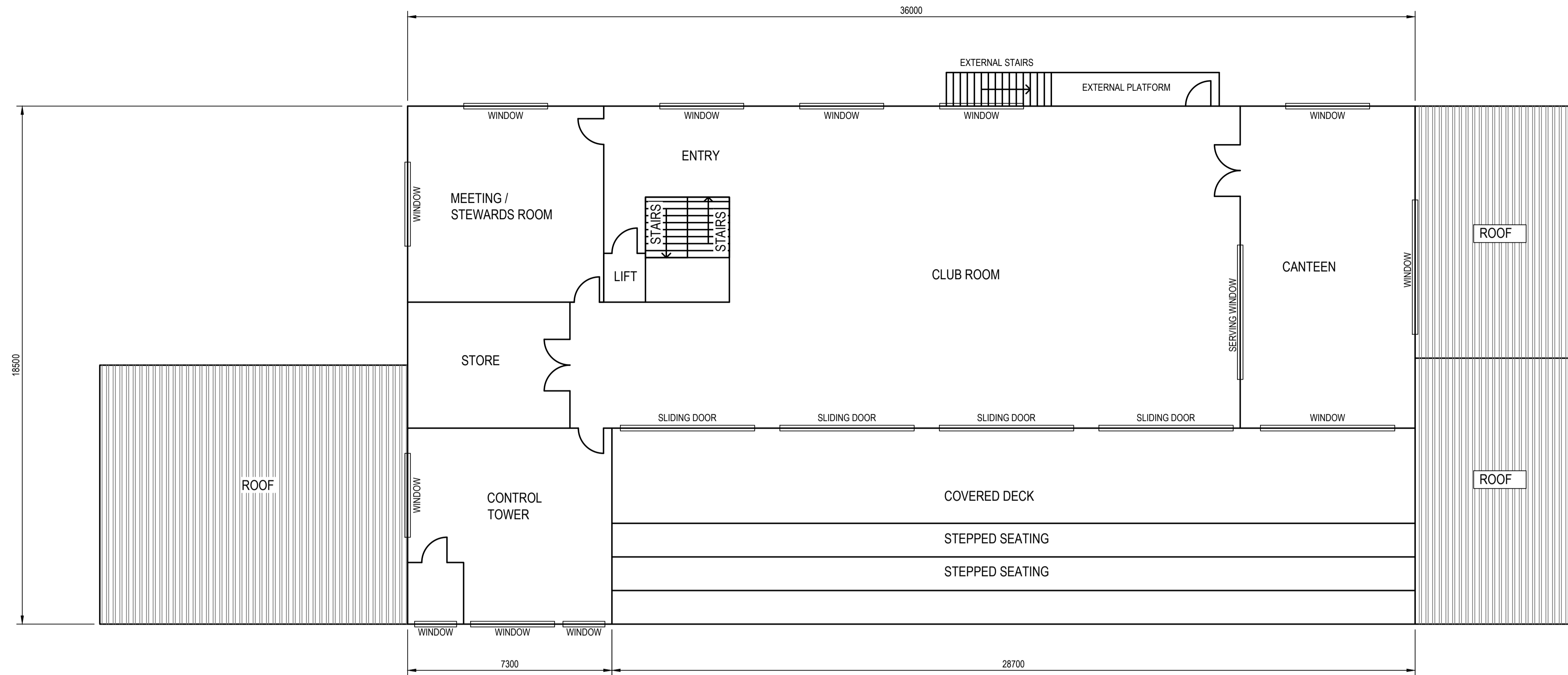
LEVEL 1 - GENERAL ARRANGEMENT
